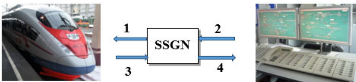
Fig. 4. Scheme for SSGN channel simulation on RWT (Akhmetov, 2019: 488) 1, 2 – control messages for MU; 3, 4- navigation information in ADCS
